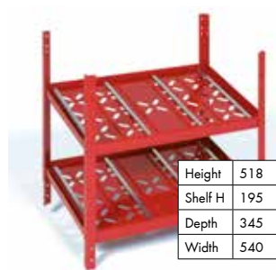
Compartment Shelf for storage boxes of size 2 Art. No. 0961 932 0
