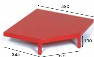
Corner Top Section Art. No. 0961 904
