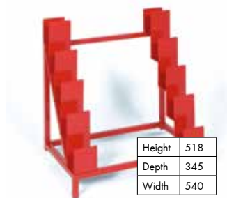
Component for threaded rods Art. No. 0961 99
