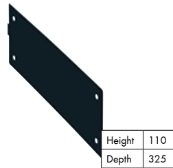
Partition Panel for double-comp. shelf Anthracite Art. No. 0961 050 043
